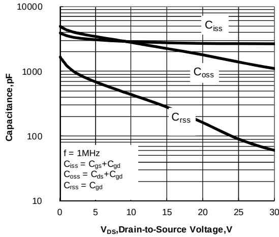
Figure 12. Capacitance Characteristics
