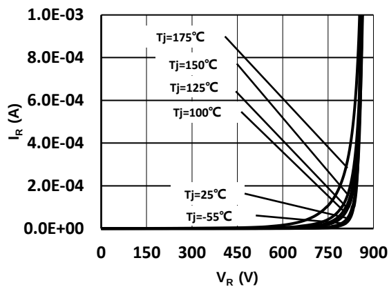
Fig 2: Reverse Characteristics
