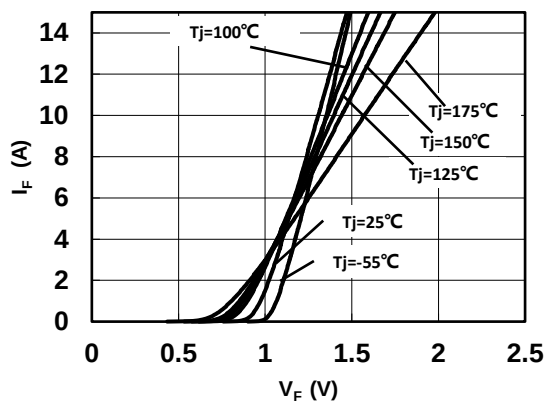
Fig 1: Forward Characteristics
