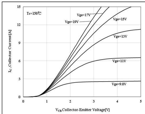
Figure 2. Output Characteristics
