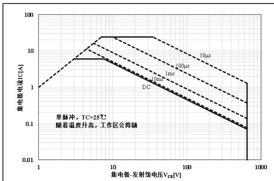
Figure 19. Forward Bias Safe Operating Area
