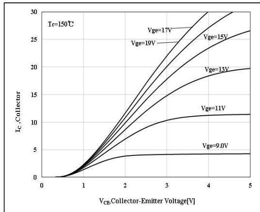
Figure 2. Output Characteristics
