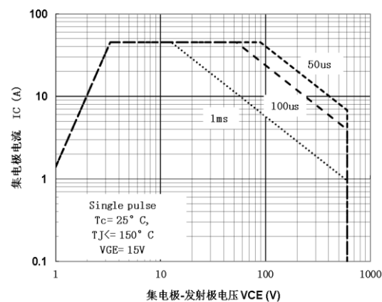
Figure 16.Forward Bias Safe Operating Area
