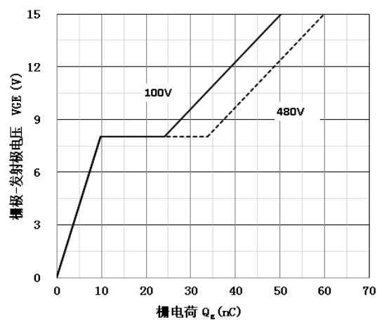
Figure 14.Gage Charge Characteristics
