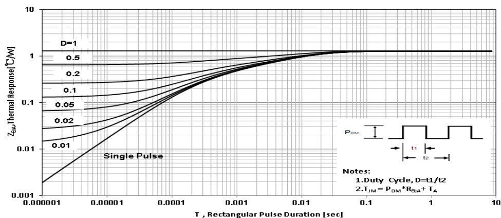
Figure 17.IGBT Transient Thermal Impedance
