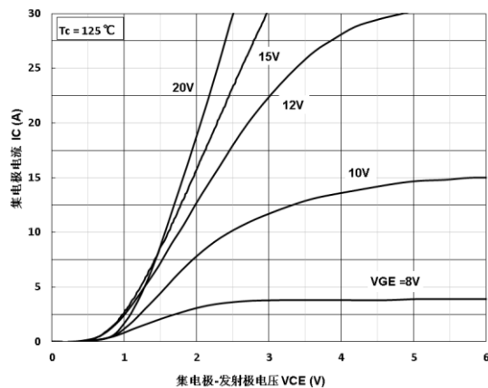
Figure 2. Output Characteristics
