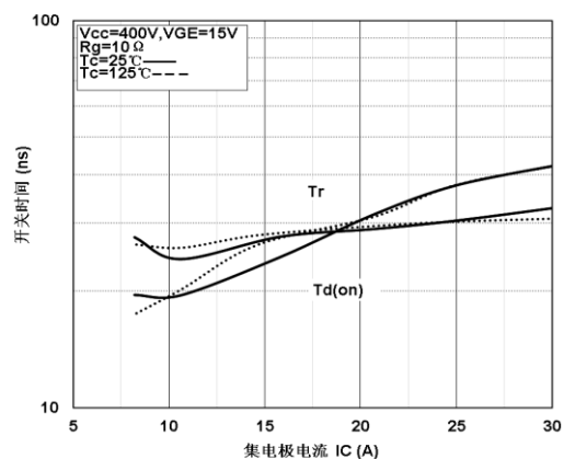
Figure 5. Switching Time - I_c Characteristics
