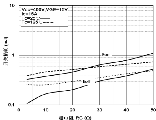
Figure 8. Switching Loss- R_g Characteristics
