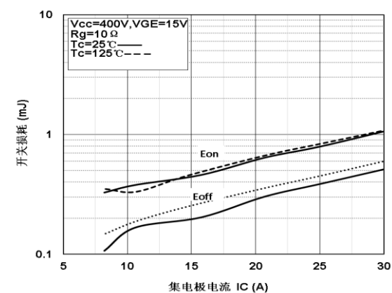
Figure 6. Switching Loss - I_c Characteristics
