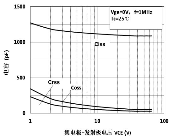
Figure 13.Capacitance Characteristics
