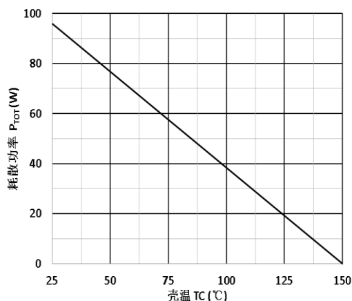
Figure 15.Power Dissipation- T_C Characteristics
