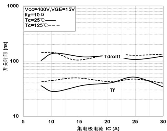
Figure 7. Switching Time - I_C Characteristics
