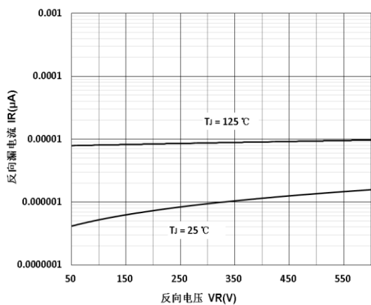
Figure 11. Diode V_R - I_R Characteristics
