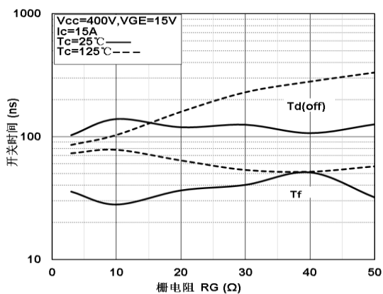
Figure 9. Switching Time- R_g Characteristics
