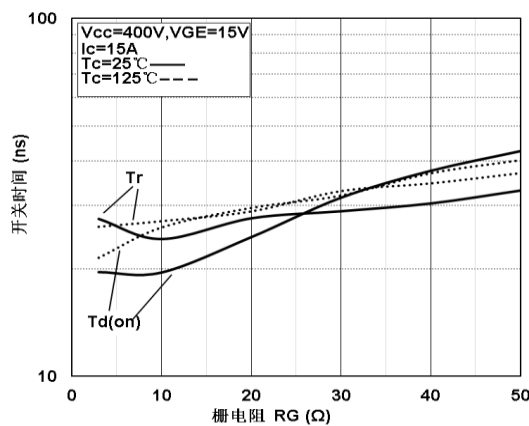
Figure 10. Switching Time- R_g Characteristics
