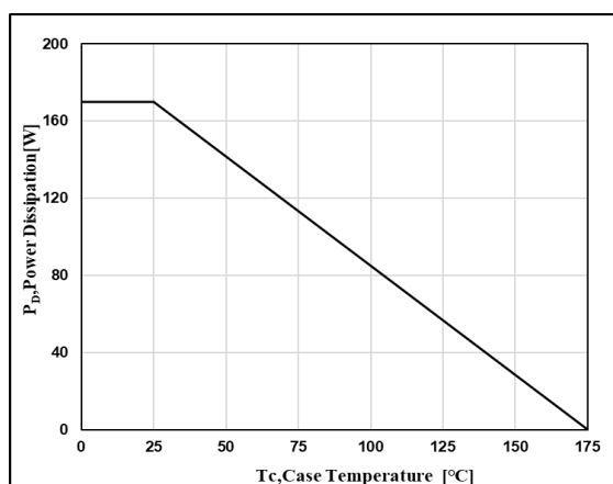
Figure 17.Power dissipation
