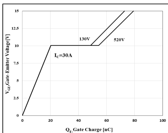
Figure 18.Gate Charge Characteristics
