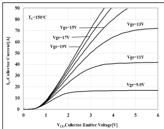
Figure 2. Output Characteristics
