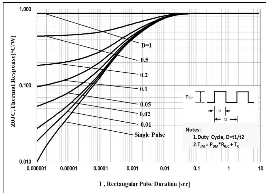
Figure 20. IGBT Transient Thermal Impedance
