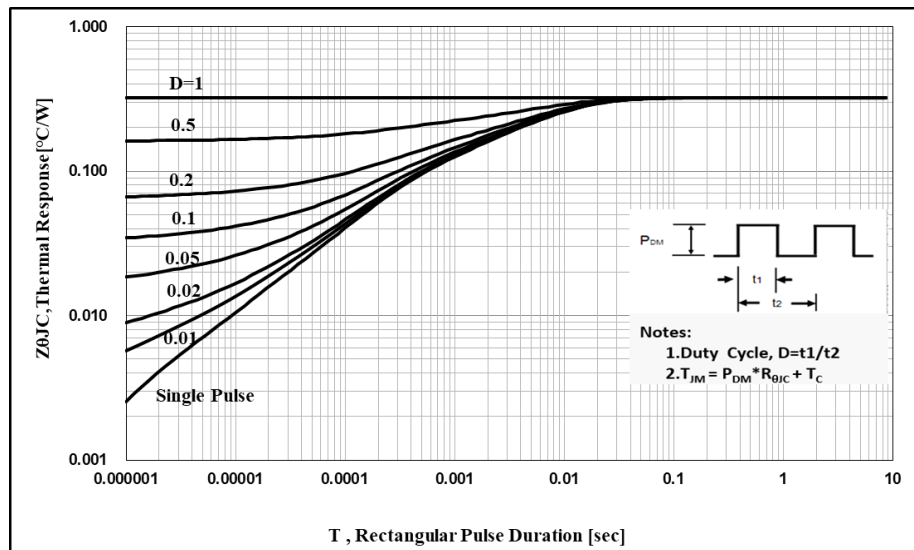
Figure 20. IGBT Transient Thermal Impedance
