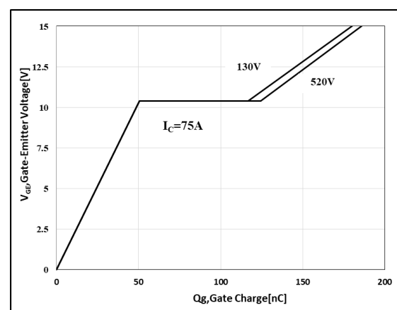
Figure 18.Gate Charge Characteristics
