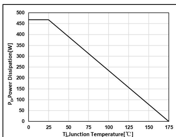
Figure 17.Power dissipation
