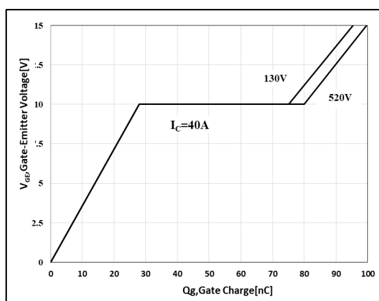
Figure 18.Gate Charge Characteristics
