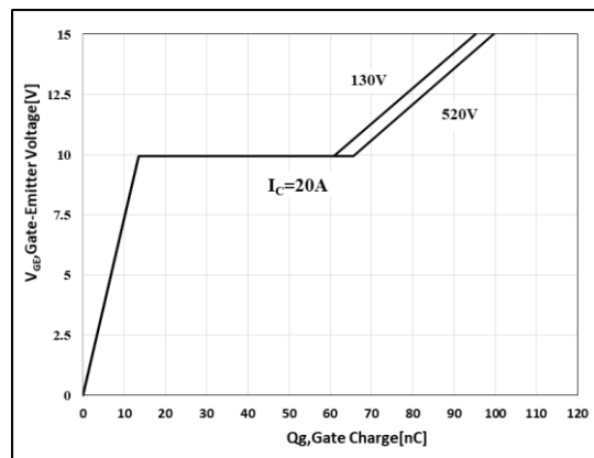
Figure 18.Gate Charge Characteristics
