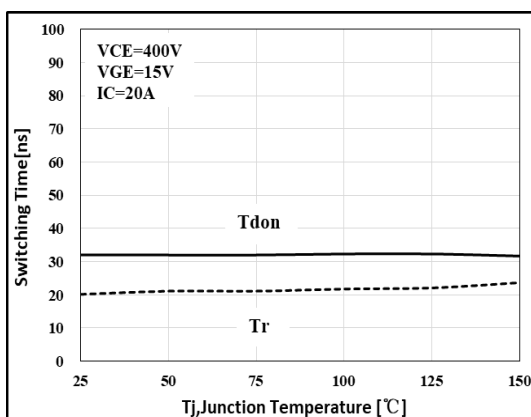
Figure 10.Switching Time- T_j Characteristics
