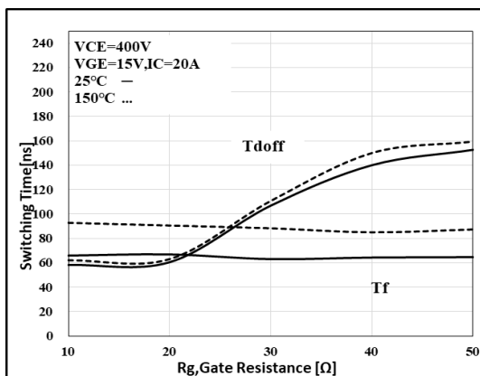
Figure 8.Switching Time- R_g Characteristics
