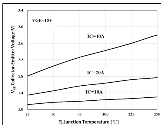
Figure 4. Saturation Voltage -Tj Characteristics
