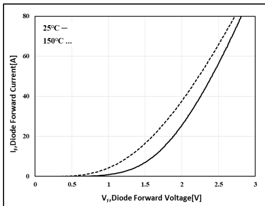
Figure 15.Diode Forward Characteristics
