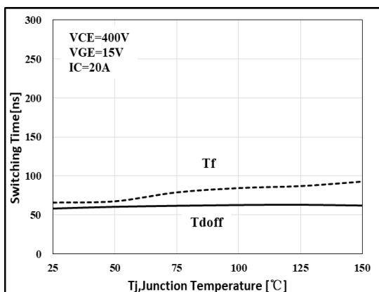
Figure 11.Switching Time- T_j Characteristics
