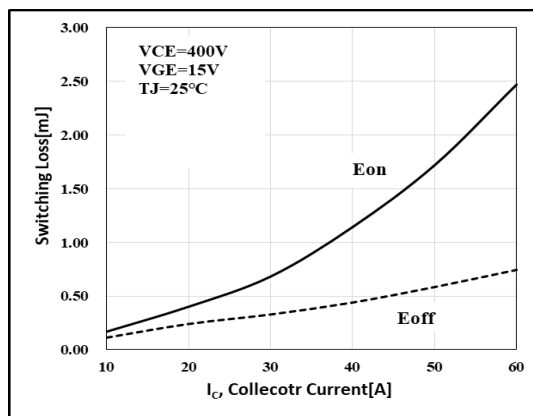
Figure 12.Switching Loss- I_C Characteristics
