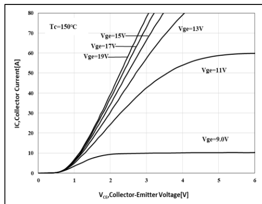
Figure 2. Output Characteristics
