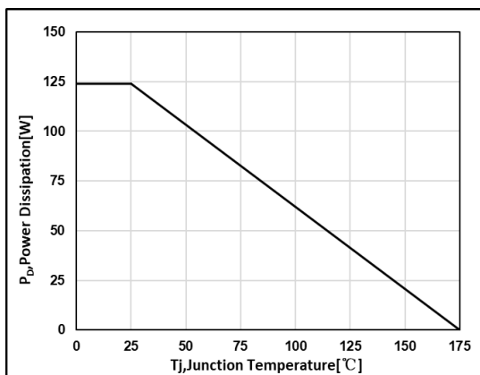
Figure 17. Power dissipation
