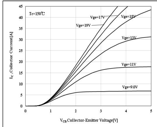
Figure 2. Output Characteristics
