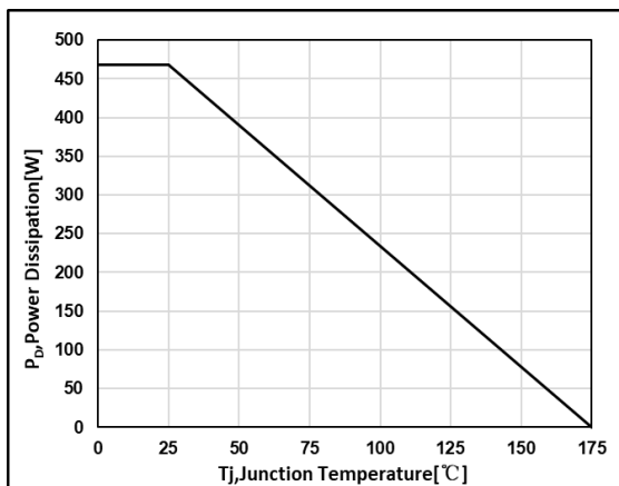
Figure 17. Power dissipation
