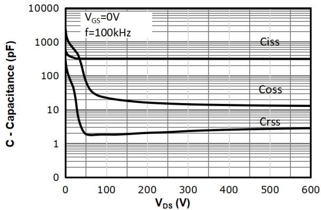
Fig 11: Capacitance Characteristics
