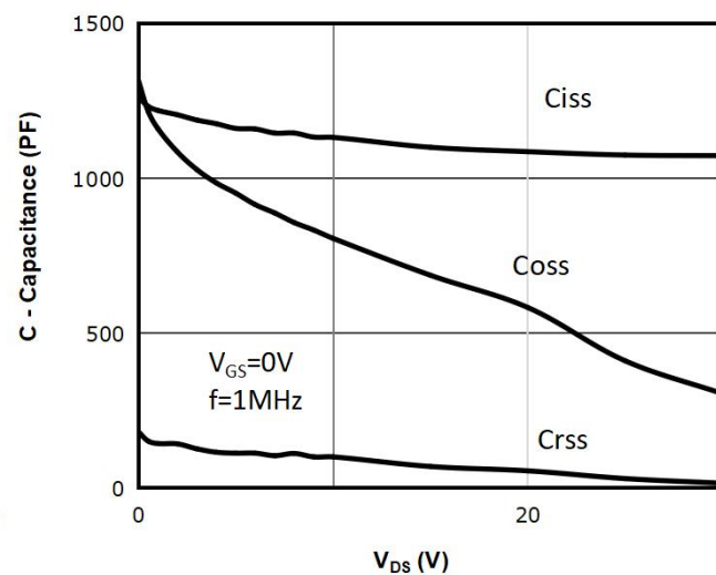
Fig 6: Capacitance Characteristics
