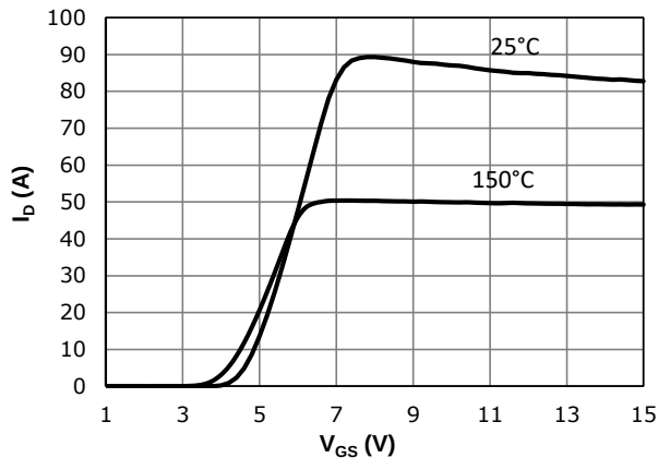
Fig 3: Transfer Characteristics
