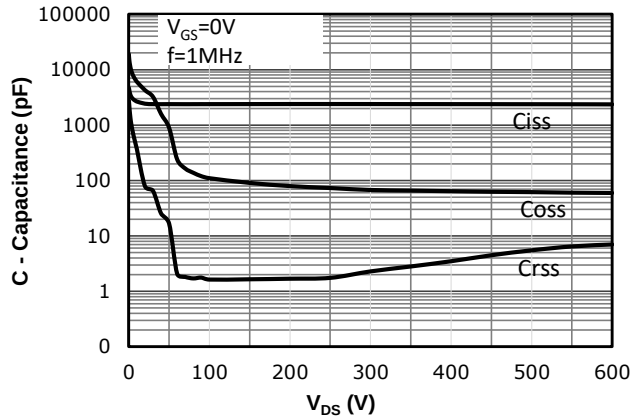
Fig 11: Capacitance Characteristics
