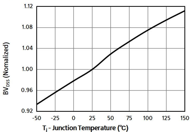
Fig 7: BV_{DS} vs. Temperature
