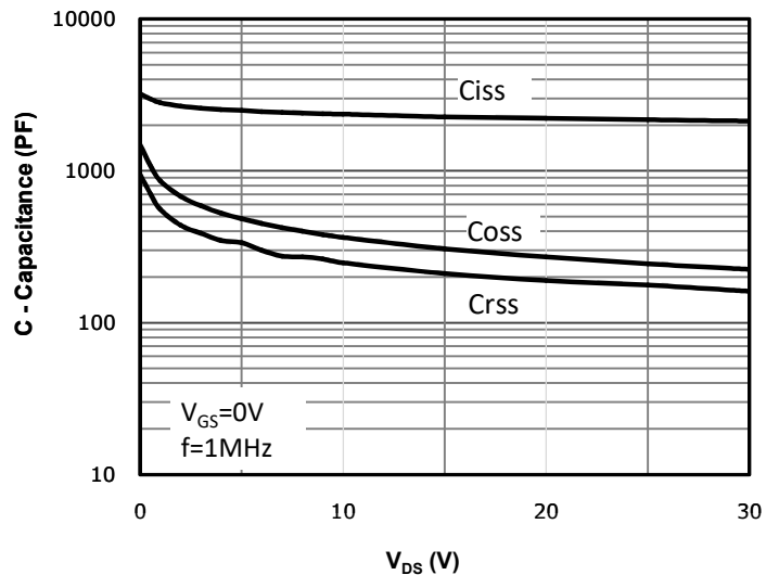
Fig 6: Capacitance Characteristics
