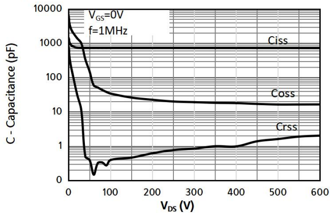
Fig 11: Capacitance Characteristics
