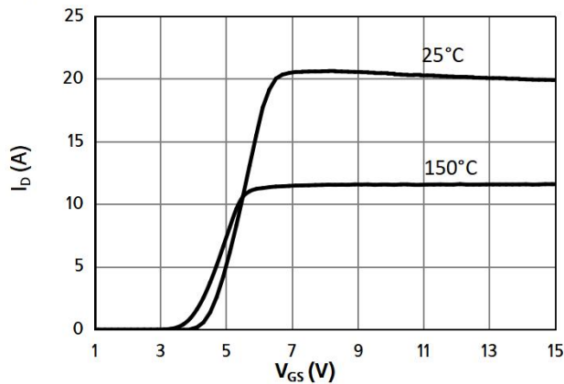
Fig 3: Transfer Characteristics
