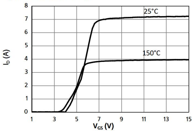
Fig 3: Transfer Characteristics
