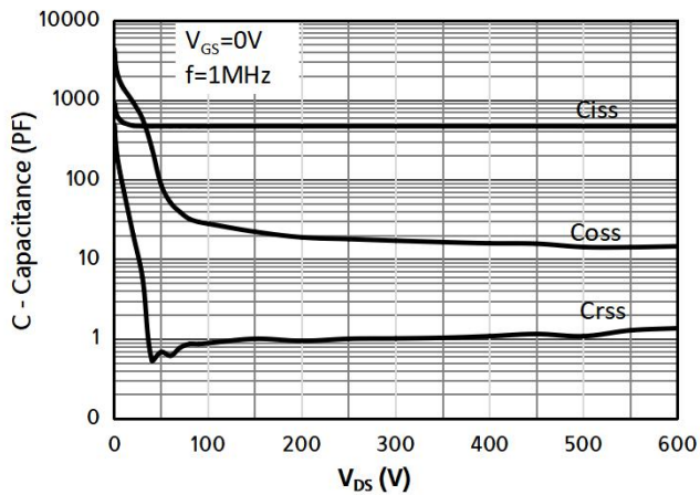
Fig 11: Capacitance Characteristics
