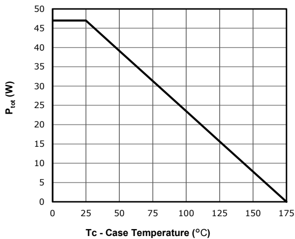
Fig 11: Power Dissipation
