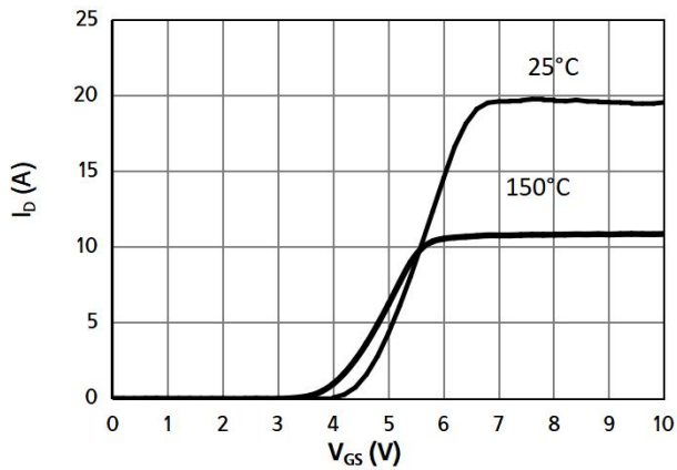
Fig 3: Transfer Characteristics
