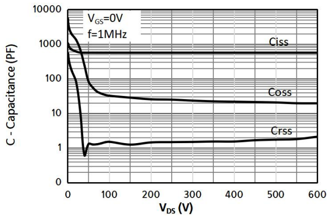
Fig 11: Capacitance Characteristics
