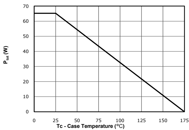
Fig 11: Power Dissipation
