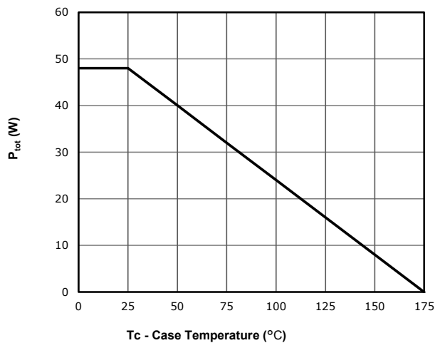
Fig 11: Power Dissipation
