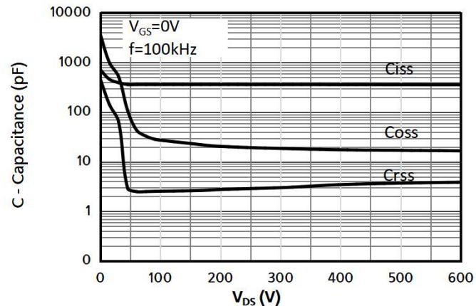
Fig 11: Capacitance Characteristics
