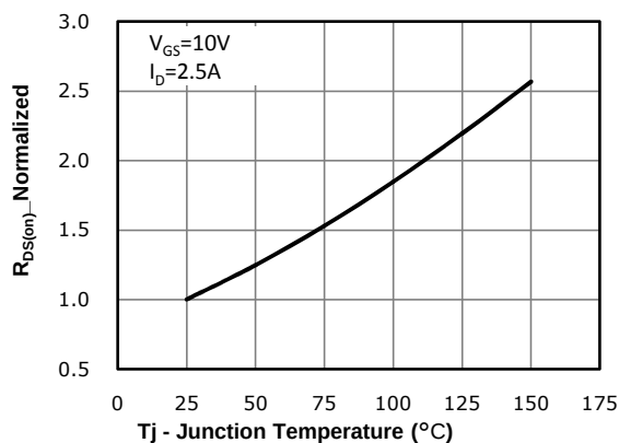
Fig 6: R_{DS(on)} vs. Temperature
