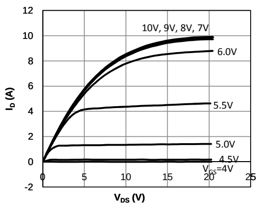
Fig 1. Output Characteristics ( T_j=25^\circ\text{C} )
