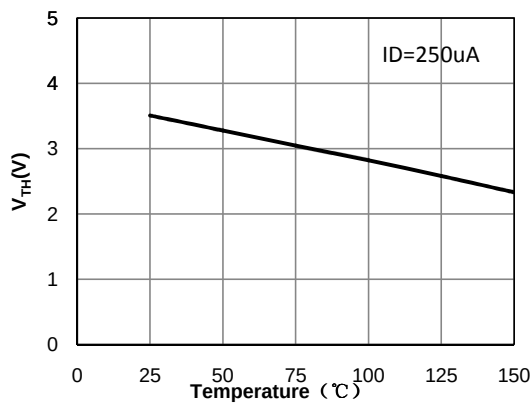
Fig 4: V_{TH} Vs T_j Temperature Characteristics
