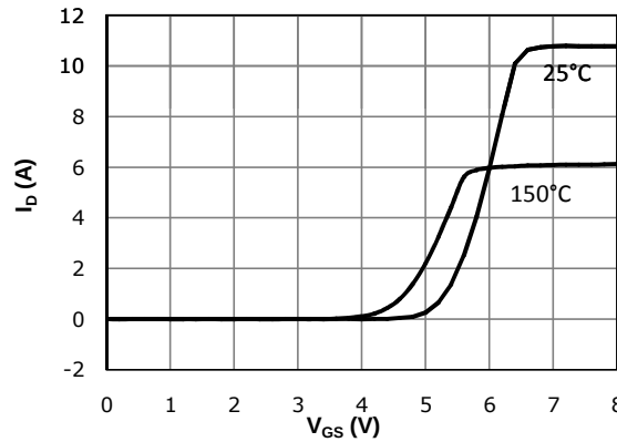
Fig 3: Transfer Characteristics
