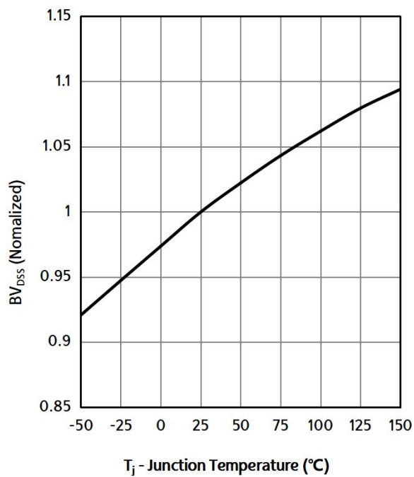
Fig 7: BV_{DSS} vs. Temperature
