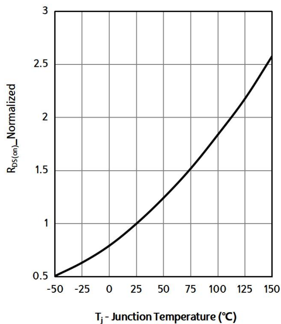
Fig 6: R_{DS(on)} vs. Temperature
