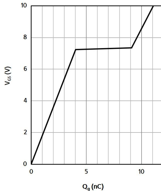
Fig 10: Gate Charge Characteristics
