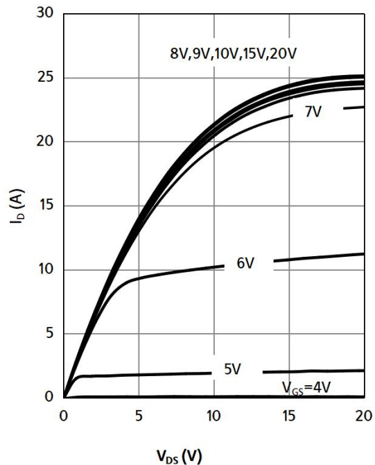
Fig 2. Output Characteristics ( T_j=150^\circ\text{C} )
