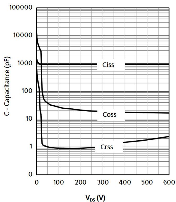
Fig 11: Capacitance Characteristics
