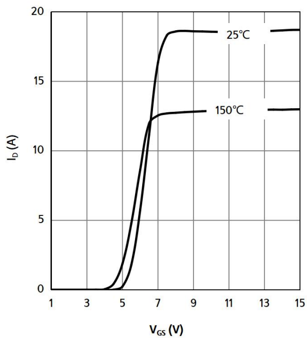
Fig 3: Transfer Characteristics
