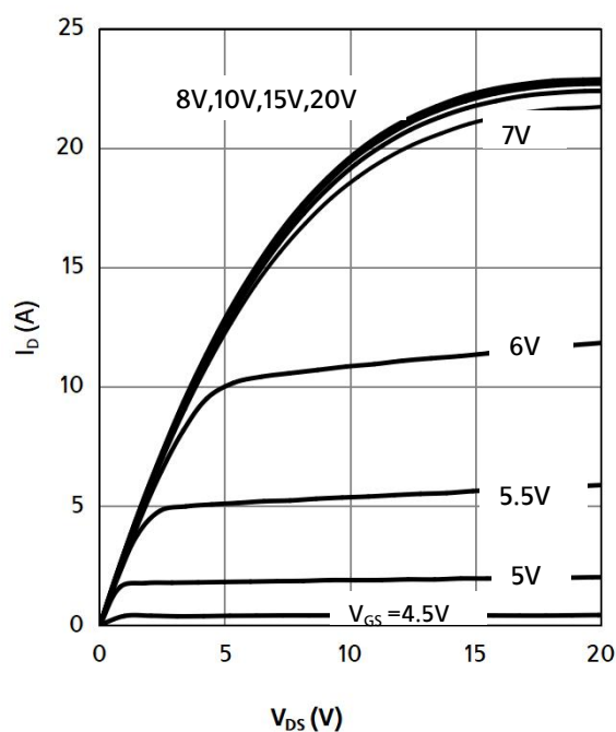
Fig 2. Output Characteristics ( T_j=150^\circ\text{C} )
