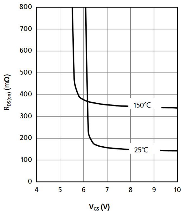
Fig 8: R_{DS(on)} vs. Gate Voltage
