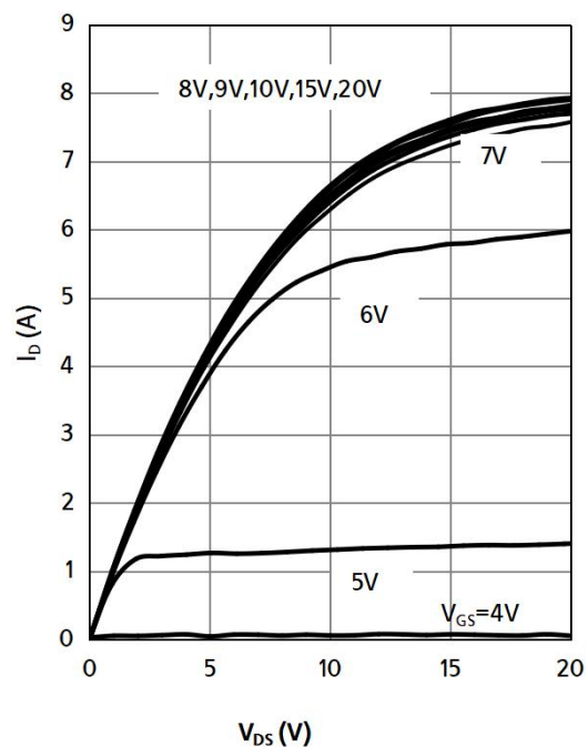
Fig 2. Output Characteristics ( T_j=150^\circ\text{C} )
