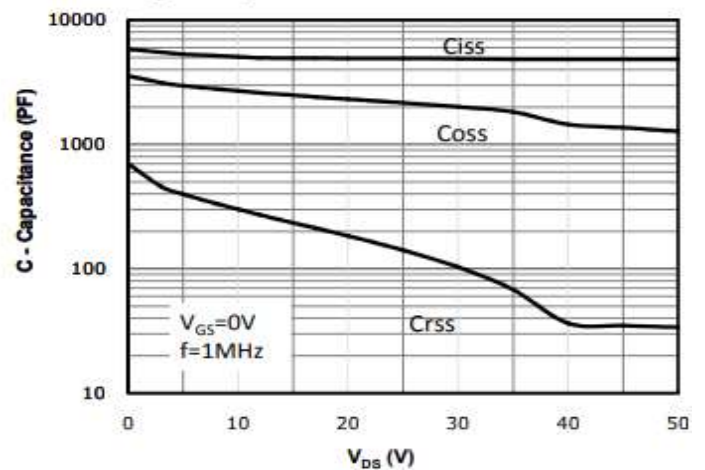
Fig 6: Capacitance Characteristics
