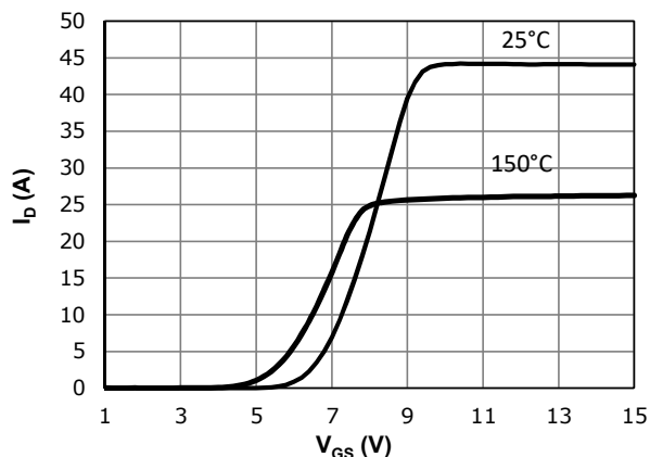
Fig 3: Transfer Characteristics
