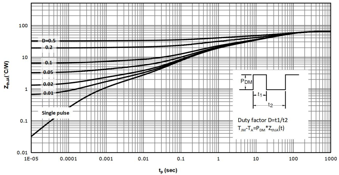
Fig 10: Max. Transient Thermal Impedance
