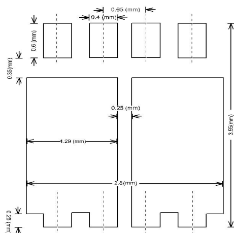
Land Pattern (Only For Reference)
