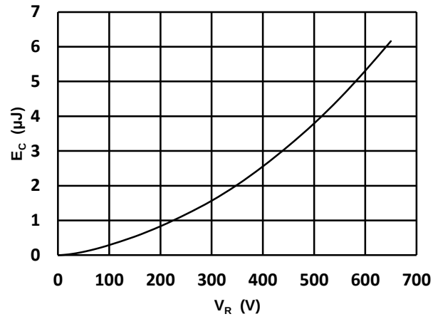
Fig 7: Typical Capacitance Stored Energy
