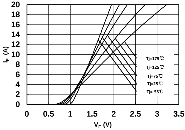
Fig 1: Forward Characteristics
