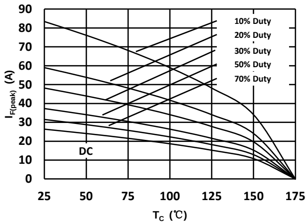
Fig 3: Current Derating
