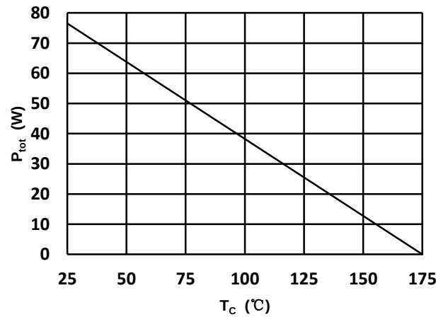
Fig 4: Power Derating
