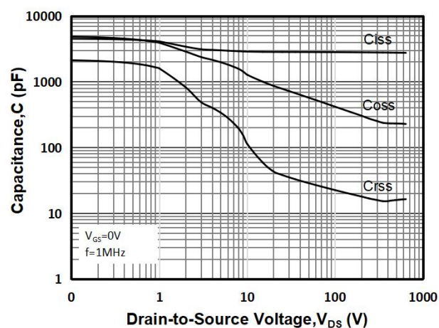
Fig 12: Capacitance Characteristics
