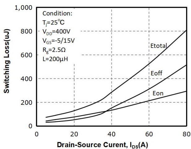
Fig 21: I_{DS}(\text{A}) vs. Switching Loss(uJ)
