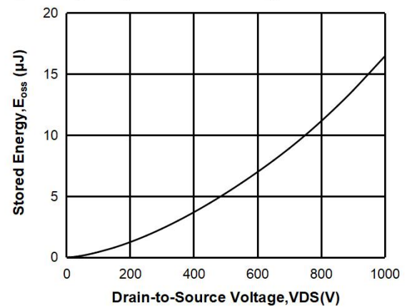
Fig 16: Output Capacitor Stored Energy
