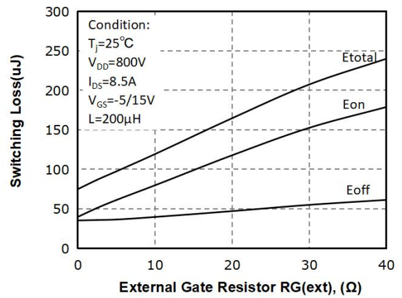
Fig 19: R_g(\Omega) vs. Switching Loss(uJ)
