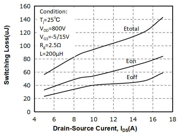
Fig 21: I_{DS}(\text{A}) vs. Switching Loss(uJ)
