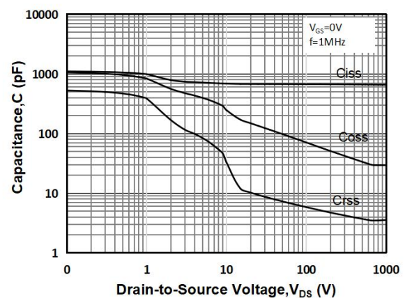
Fig 12: Capacitance Characteristics
