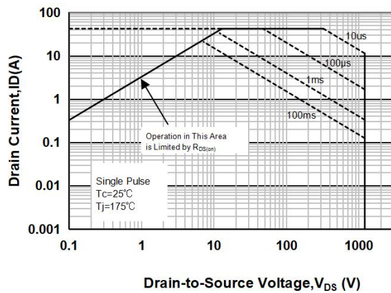
Fig 15: Safe Operating Area
