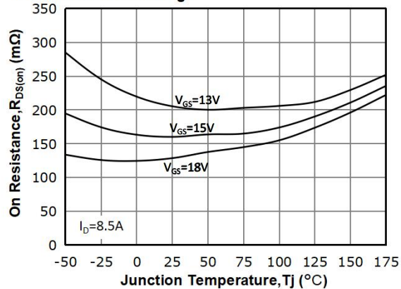
Fig 6: R_{DS(on)} vs. Temperature For Various Gate Voltage
