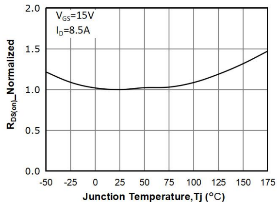
Fig 4: R_{DS(on)} vs. Temperature
