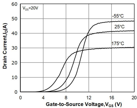
Fig 7: Transfer Characteristics
