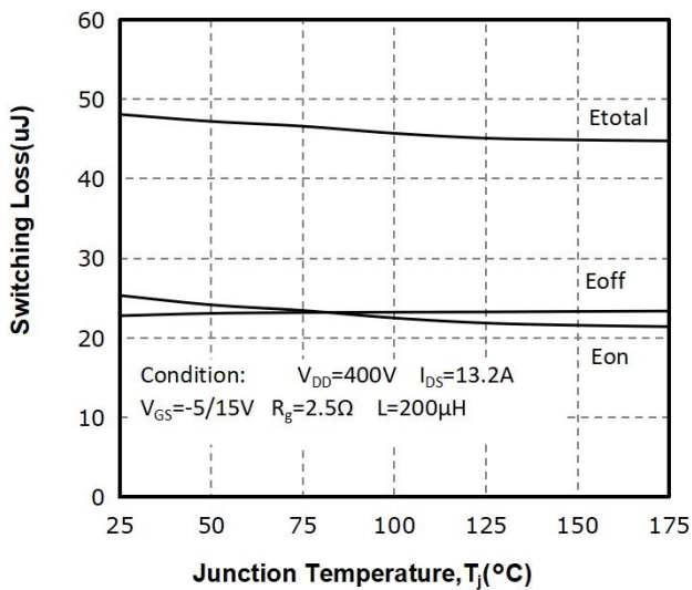
Fig 20: Temperature( ^\circ\text{C} ) vs. Switching Loss(uJ)
