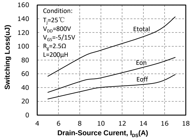
Fig 21: I_{DS}(\text{A}) vs. Switching Loss(uJ)
