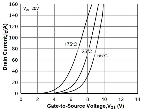
Fig 7: Transfer Characteristics
