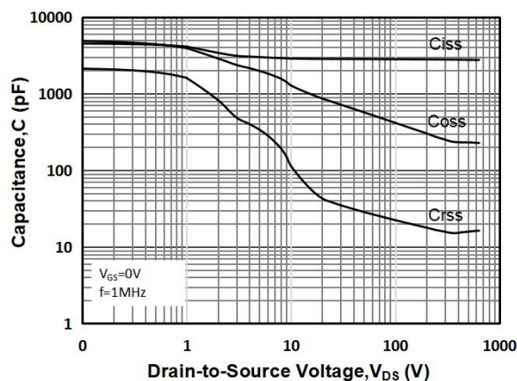
Fig 12: Capacitance Characteristics
