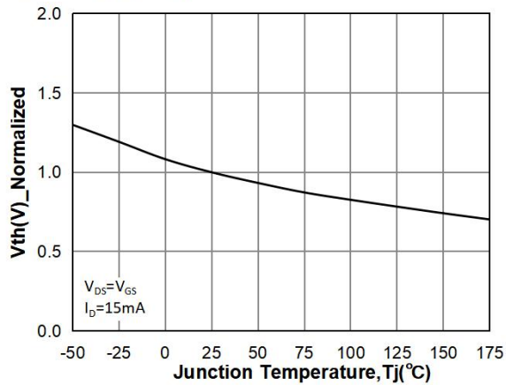
Fig 9: V_{th}(th) Vs T_j Characteristics
