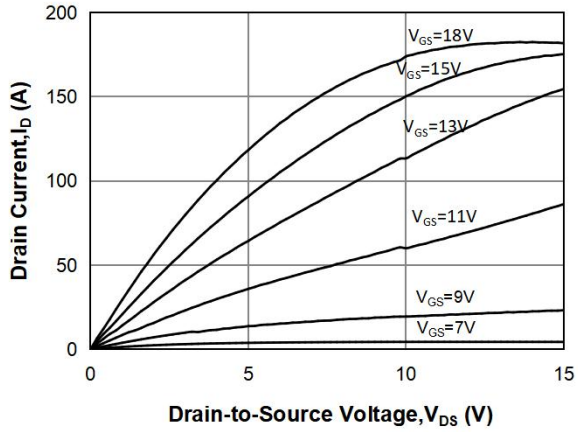
Fig 1. Output Characteristics ( T_J = -55^\circ\text{C} )
