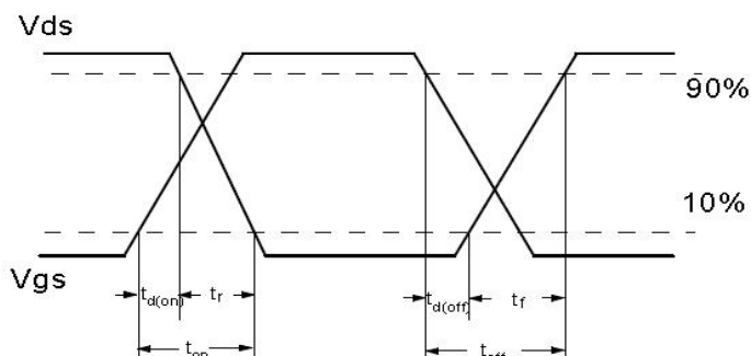
Resistive Switching Test Circuit &amp; Waveforms
