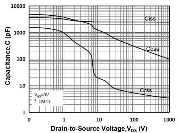
Fig 12: Capacitance Characteristics
