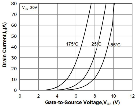
Fig 7: Transfer Characteristics
