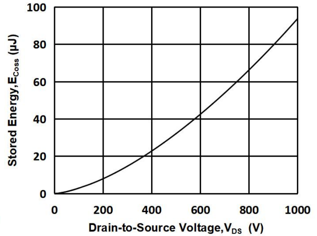
Fig 16: Output Capacitor Stored Energy
