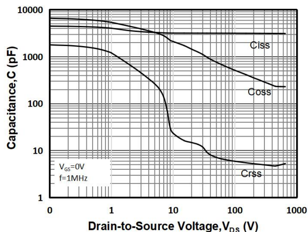
Fig 12: Capacitance Characteristics
