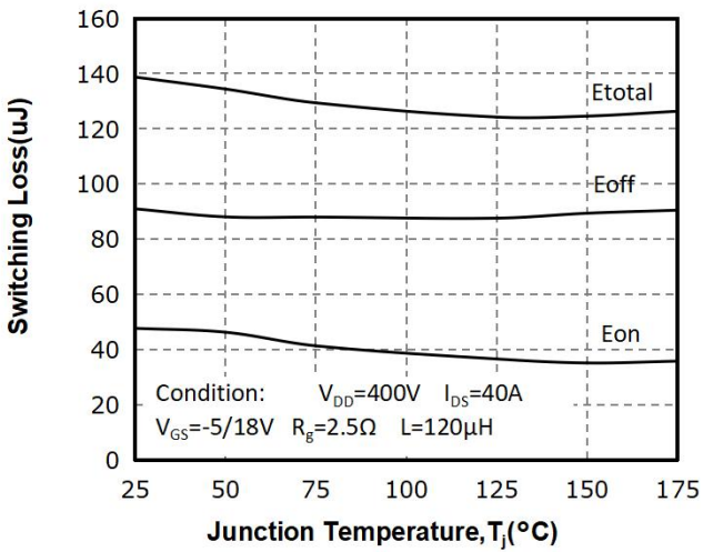
Fig 20: Temperature(°C) vs. Switching Loss(uJ)
