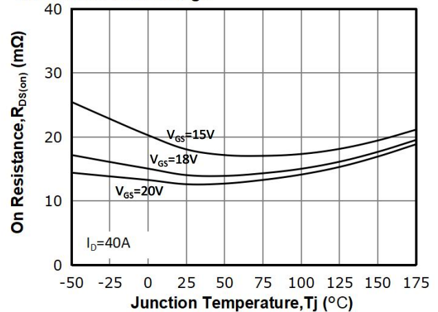
Fig 6: R_{DS(on)} vs. Temperature For Various Gate Voltage
