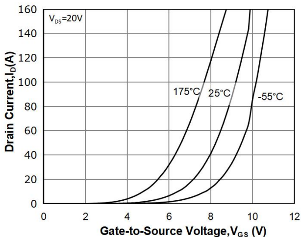
Fig 7: Transfer Characteristics
