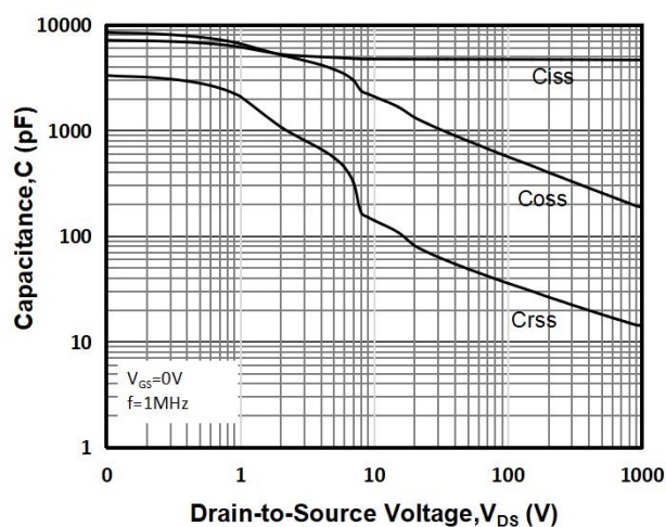
Fig 12: Capacitance Characteristics
