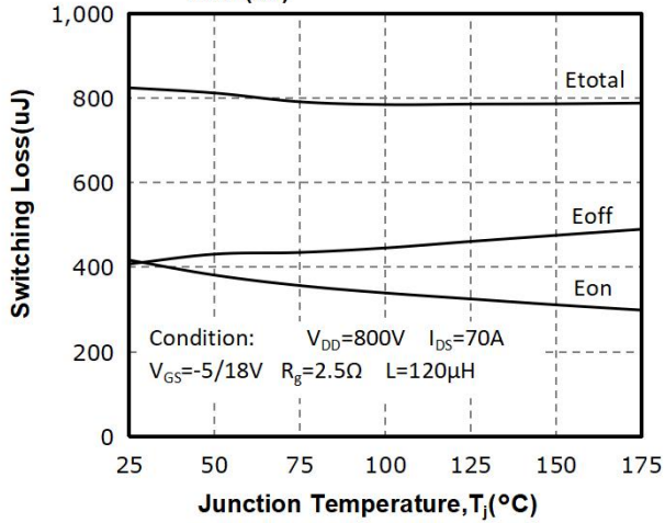
Fig 20: Temperature( ^\circ\text{C} ) vs. Switching Loss(uJ)
