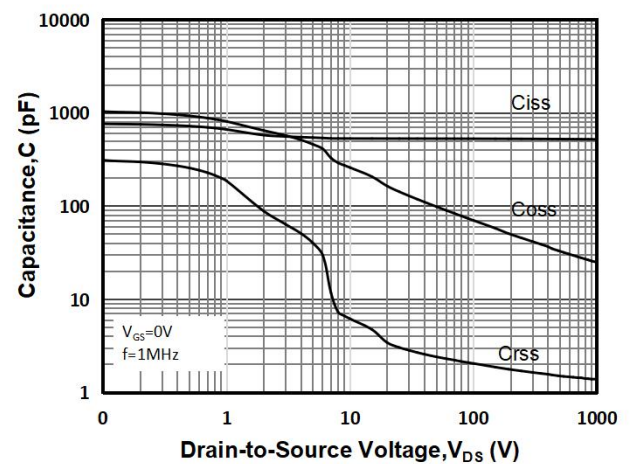
Fig 12: Capacitance Characteristics
